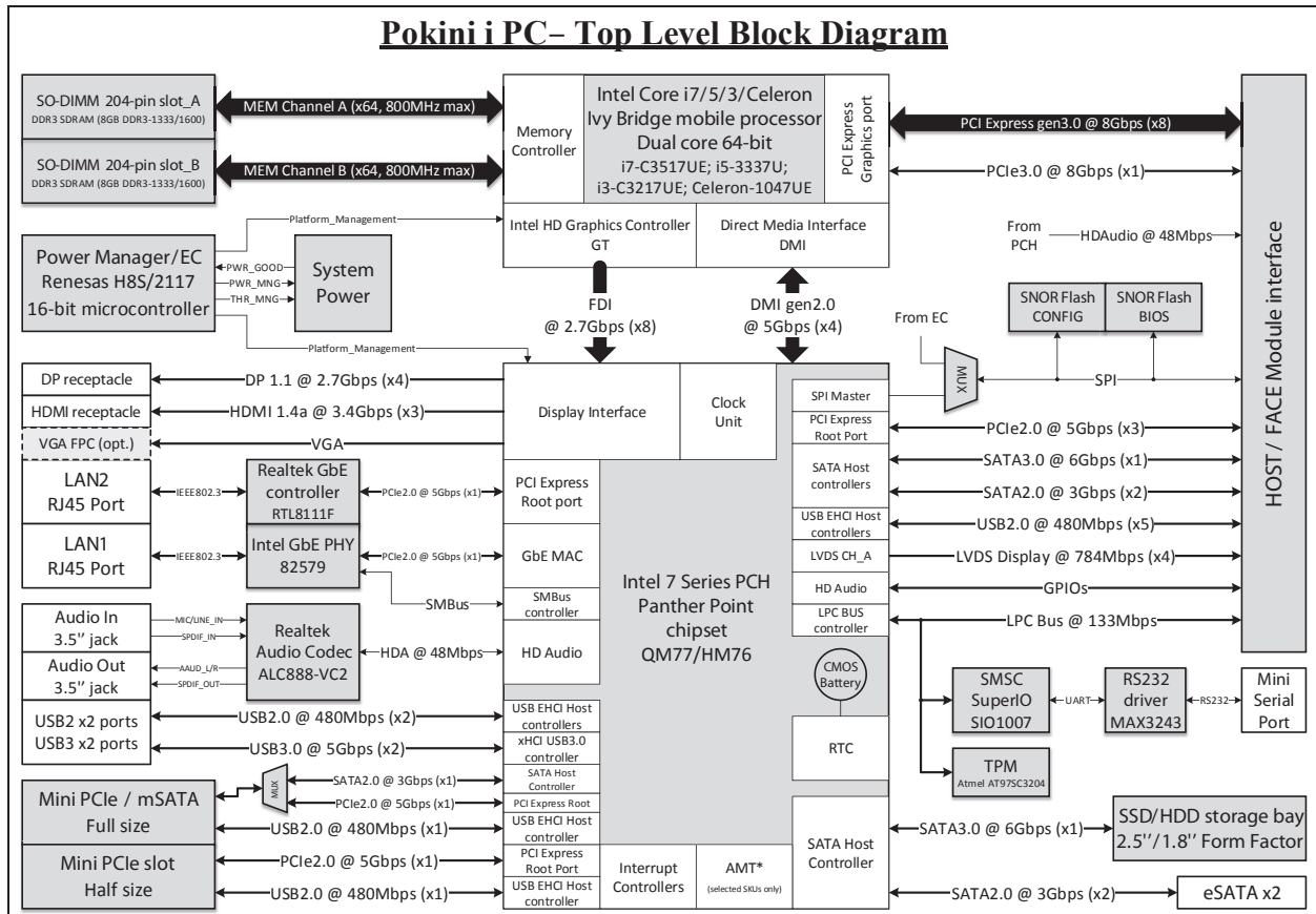
Figure 1 – Pokini i PC Top Level Block Diagram
